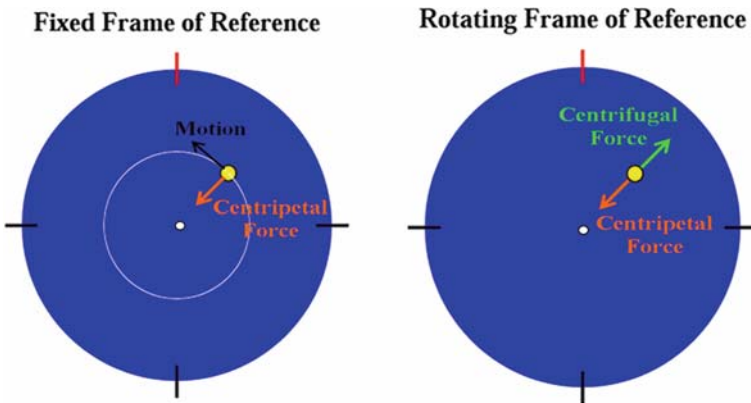
Fig. 3.13 Left panel In the fixed frame of reference, an object attached to a rope and rotating at the same rate as the turntable experiences only the centripetal force. Right panel : The object appears stationary in the rotating frame of reference, which implies a balance between the centripetal force and the centrifugal force. The SciLab script “Centripetal Force.sce” in the folder “Miscellaneous/Coriolis Force” of the CD-ROM produces an animation
