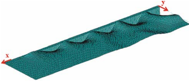
Fig. 6.1 Exercise 15. Snapshot of the deformation of the sea surface caused by a coastal Kelvin wave in the northern hemisphere
