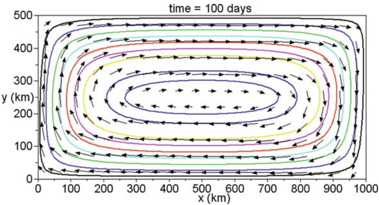
Fig. 6.16 Exercise 18. Scenario 1. Flow field (arrows, averaged over 5 \times 5 grid cells) and contours of sea-level elevation (solid lines) after 100 days of simulation. Maximum sea-level elevation is 3 cm. Maximum flow speed is 4 cm/s
