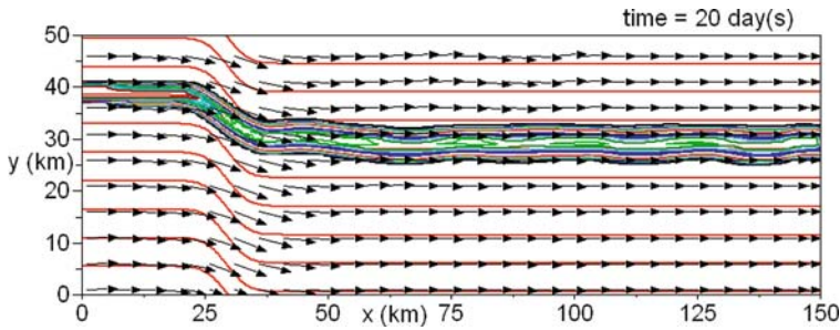
Fig. 6.5 Exercise 16. Scenario 1. Snapshot of flow field (arrows, averaged over 5 \times 5 grid cells) and Eulerian tracer concentration (crowded lines) after 20 days of simulation. Bathymetric contours are overlaid
