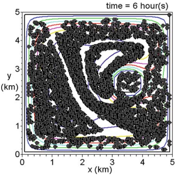
Fig. 5.13 Exercise 12. Snapshot of the locations of 3000 Lagrangian float after 6 h of simulation
