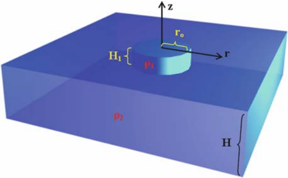
Fig. 6.20 Illustration for the description of the geostrophic adjustment process
