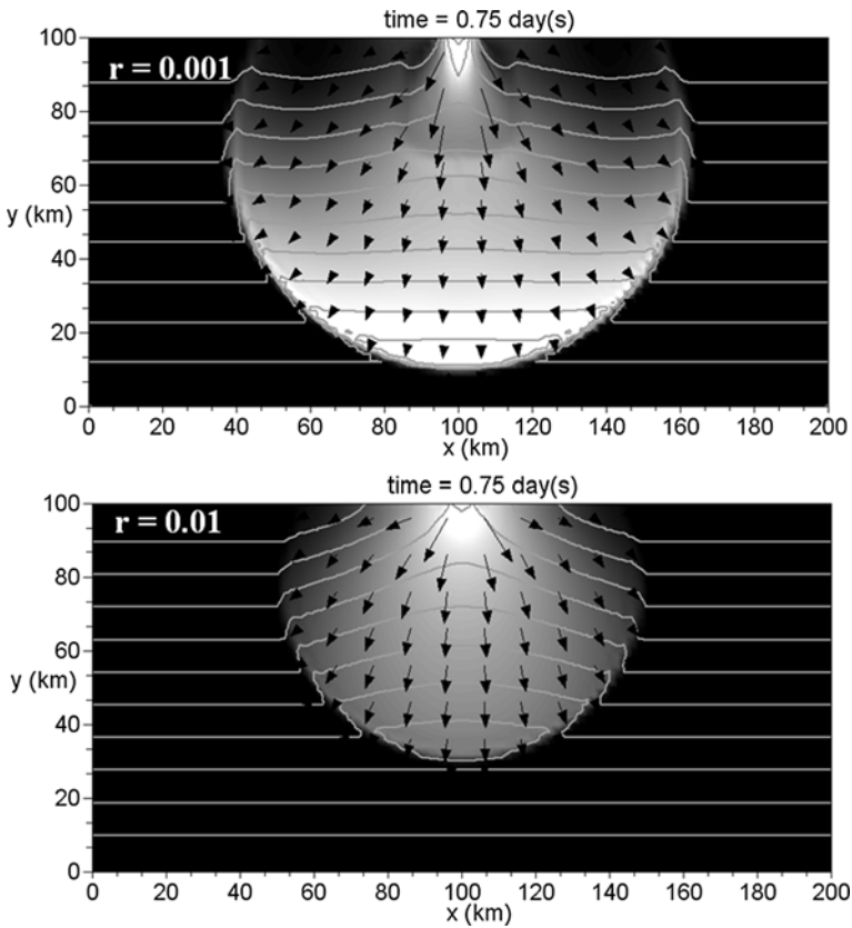
Fig. 6.31 Exercise 22. Scenario 1. Snapshots of the horizontal distribution of plume thickness (shading) for different values of the bottom-friction parameter r . The range shown is h_2 = 0 (black shading) to h_2 = 50 m (white shading). Superimposed are horizontal flow vectors (arrows, averaged over 5 \times 5 grid cells) and contours of \eta_2
