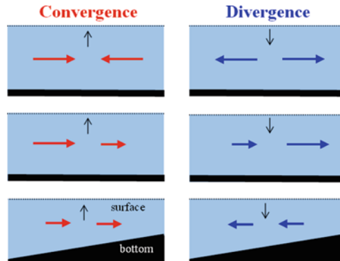
Fig. 3.7 Sketches of different flow field leading to either lateral convergence or divergence of depth-averaged horizontal fl w. Vertical arrows indicate the instant response of the sea surface
