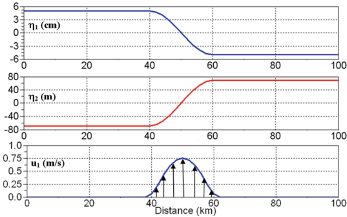
Fig. 6.25 Exercise 21. Initial distributions across the front of ( top panel ) sea-level elevation (cm), ( middle panel ) interface displacement, and ( bottom panel ) and geostrophic frontal fl w
