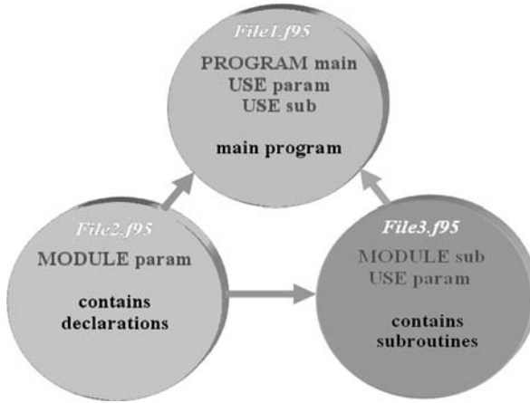
Fig. 4.8 Structure of the FORTRAN code for the following exercises
