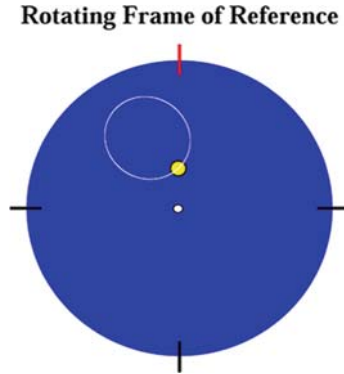
Fig. 3.18 Pathway of an object that experiences the Coriolis force in a clockwise rotating fluid. The SciLab script “Coriolis Force Revealed.sce” in the folder “Miscellaneous/Coriolis Force” of the CD-ROM produces an animation
