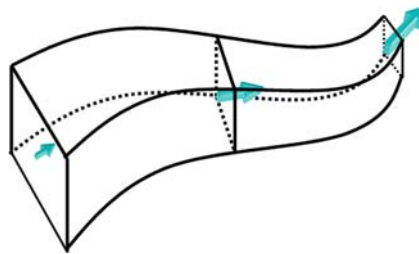
Fig. 3.8 Sketch of volume conservation in river fl ws. The fl w speed increases in sections where the cross-sectional area of the river decreases
