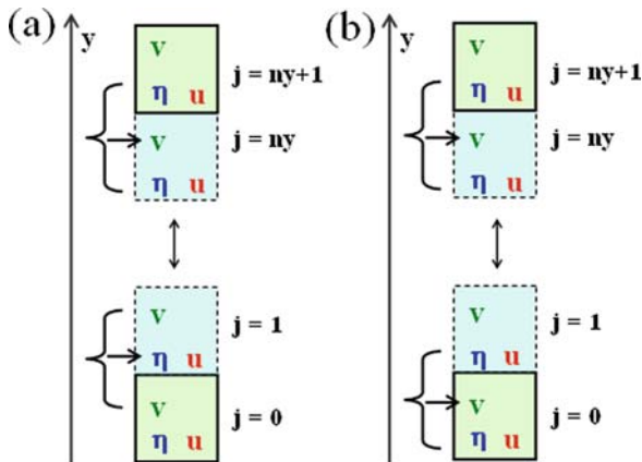
Fig. 5.5 Boundary points that need to be specific in the numerical code. In (a) v is predicted from j = 1 to j = ny , whereas in (b) the prediction loop includes j = 0
