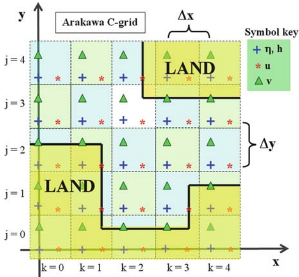
Fig. 5.2 Example of land and coastlines in the Arakawa C-grid
