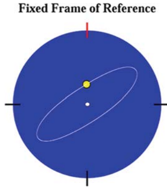
Fig. 3.16 Trajectory of motion (white line) for one complete revolution of a clockwise rotating fluid tank as seen in the fixed frame of reference. The SciLab script “Traject” in the folder “Miscellaneous/Coriolis Force” of the CD-ROM produces an animation
