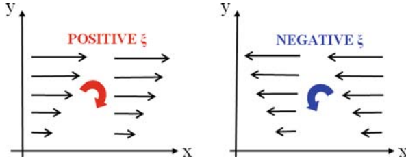
Fig. 6.2 Examples of horizontal fl w f elds exhibiting positive or negative relative vorticity
