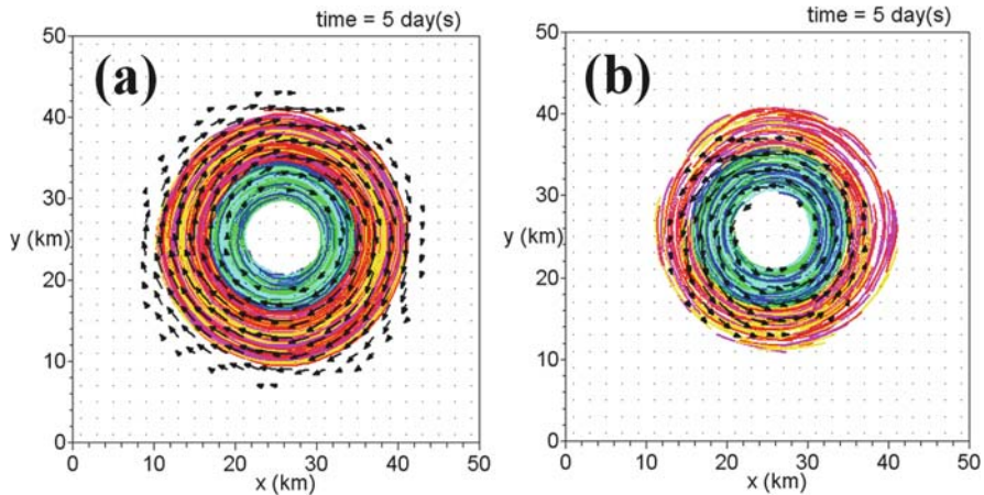
Fig. 6.24 Exercise 20. Flow field (arrows) in the (a) surface and (b) bottom layers after 5 days of simulation. Maximum flow speed in the surface layer is 33 cm/s and in the bottom layer this is 10 cm/s. Velocity vectors are averaged over 2 \times 2 grid cells. Curves are trajectories of 400 Lagrangian float predicted over the last 3 days of simulation
