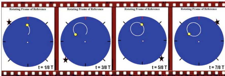
Fig. 3.24 Snapshots of the trajectory (white line) of a water parcel subject to the Coriolis force as predicted with the semi-implicit approach. The star denotes a reference location in the fixed frame of reference
