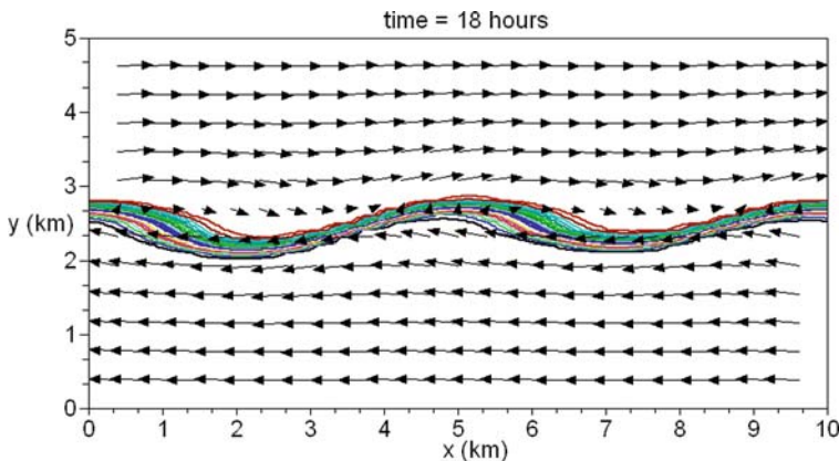
Fig. 6.8 Exercise 17. Development of wavy disturbances on a shear-fl w profile. Shown are tracer concentration ( contours ) and fl w vectors ( arrows ) after 18 h of simulation. Flow vectors are averaged over 3 \times 3 grid cells
