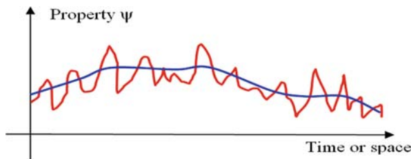
Fig. 3.26 Observed values of a physical property (wiggly line) can be expressed in terms of a mean value (smooth line), averaged over a certain time and/or space interval, plus fluctuations (difference between both lines)
