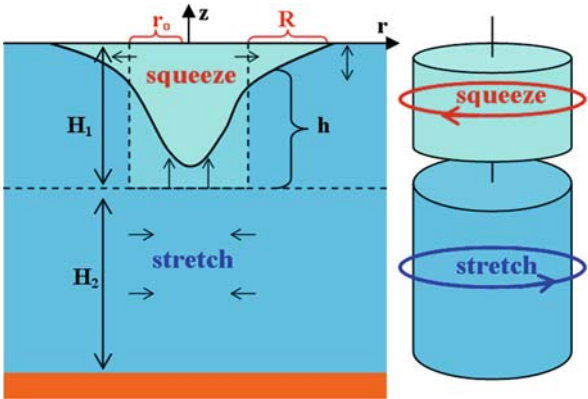
Fig. 6.21 Illustration of the geostrophic adjustment process in a 2-layer ocean and resultant geostrophic eddies for the northern hemisphere
