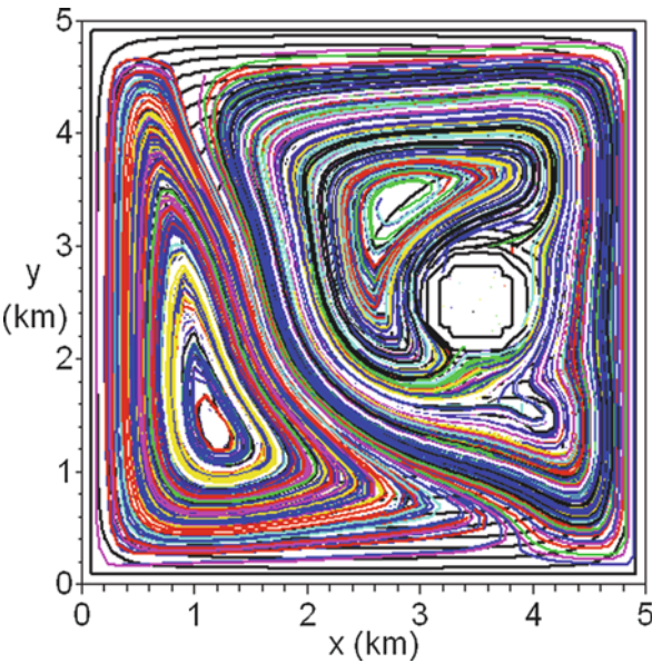
Fig. 5.14 Exercise 12. Trajectories of 500 Lagrangian float over 12 h of simulation
